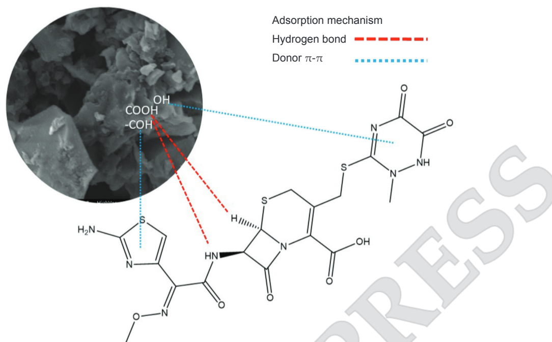
Figure 6. Proposed adsorption mechanism of ceftriaxone as a model antibiotics residue in this study to activated carbon from PKM.
