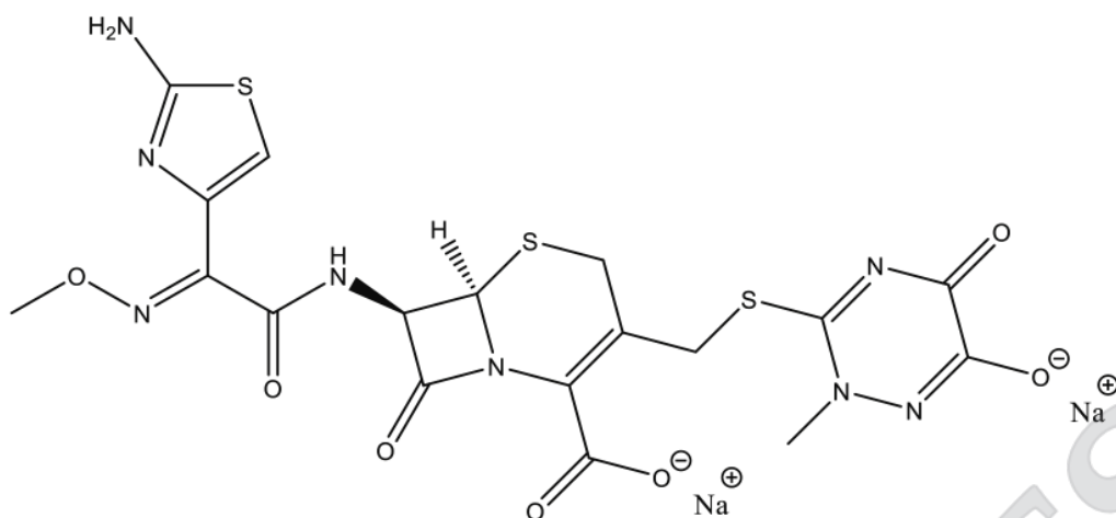
Figure 1. Structure of sodium ceftriaxone.
