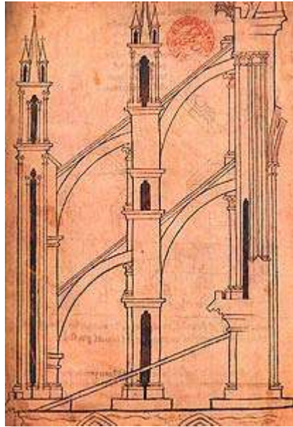
Villard de Honnecourt's drawing of a flying buttress at Reims, ca. AD 1320–1335 (Bibliothèque nationale)
