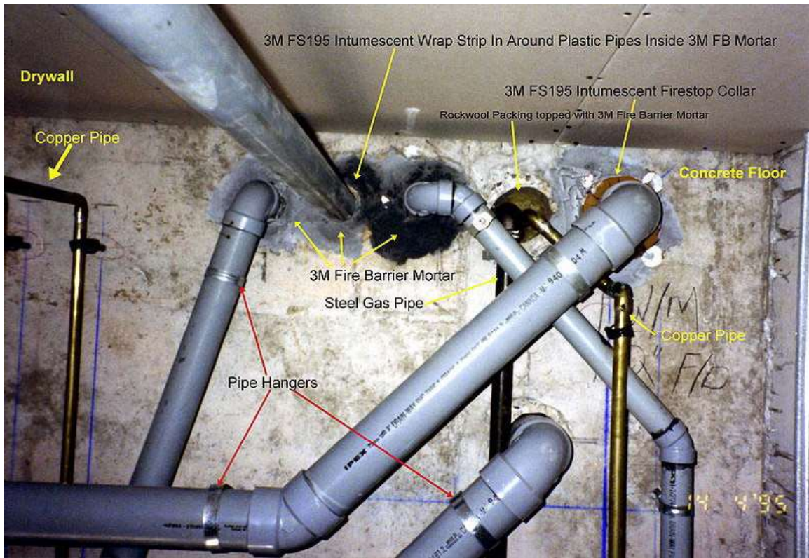
Plastic pipes penetrating a concrete floor in a Canadian highrise apartment building
