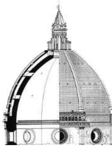
Section and elevation of Brunelleschi's dome
