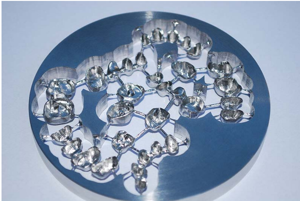
Chrome-cobalt disc with bridges and crowns for dental implants manufactured using WorkNC Dental CAD/CAM
