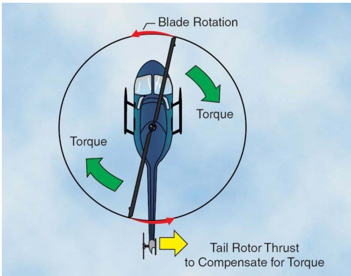
Antitorque: Torque effect on a helicopter
