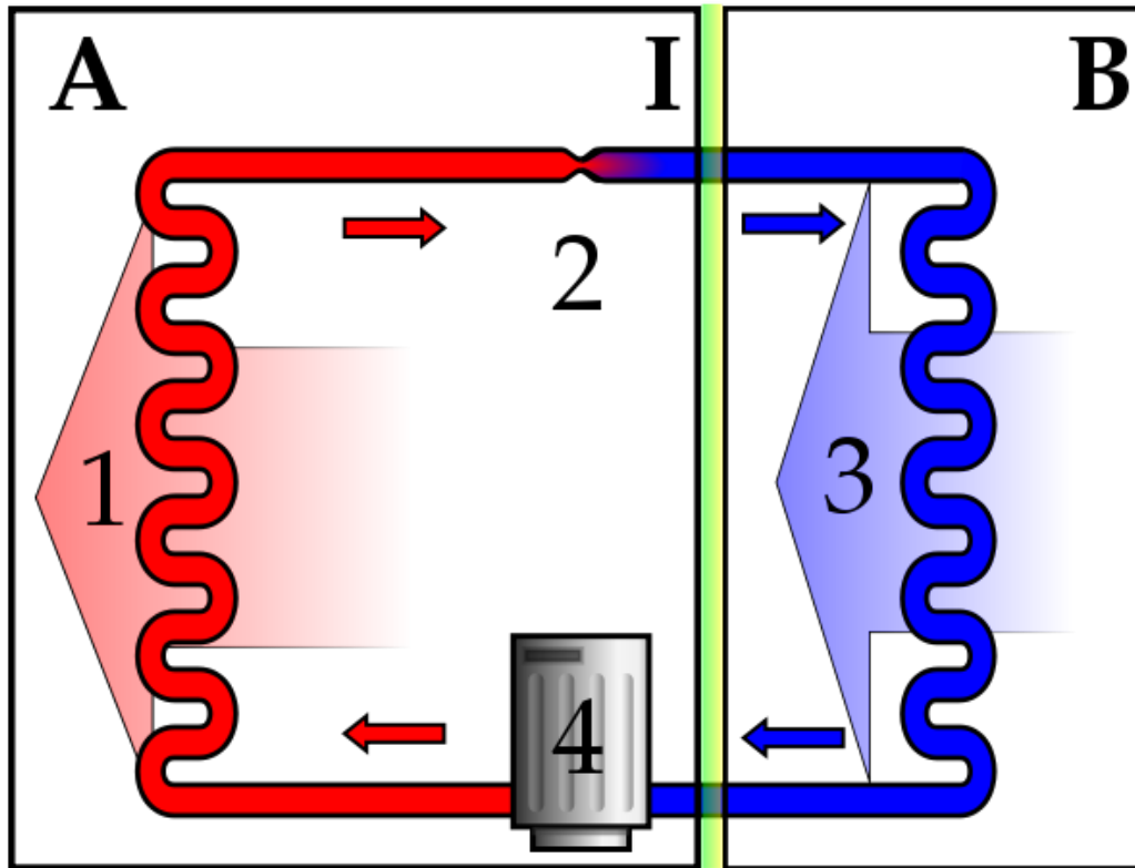
A: indoor compartment, B: outdoor compartment, I: insulation, 1: condenser, 2: expansion valve, 3: evaporator, 4: compressor
