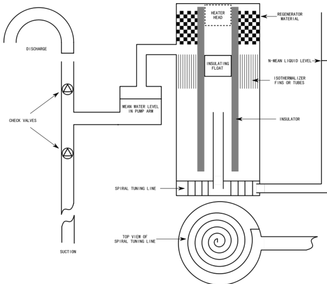
A Concentric-cylinder Fluidyne Pumping engine
