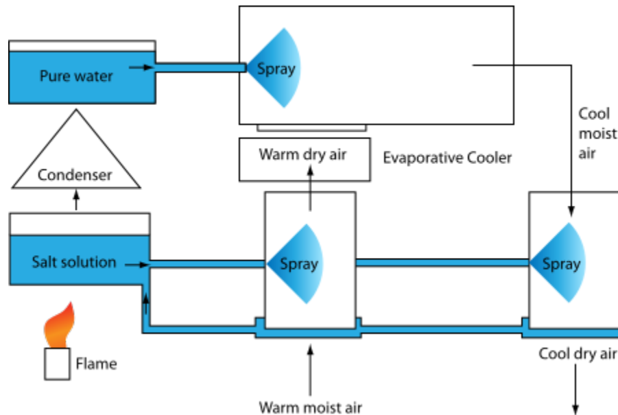
Water Spray Absorption Refrigeration
