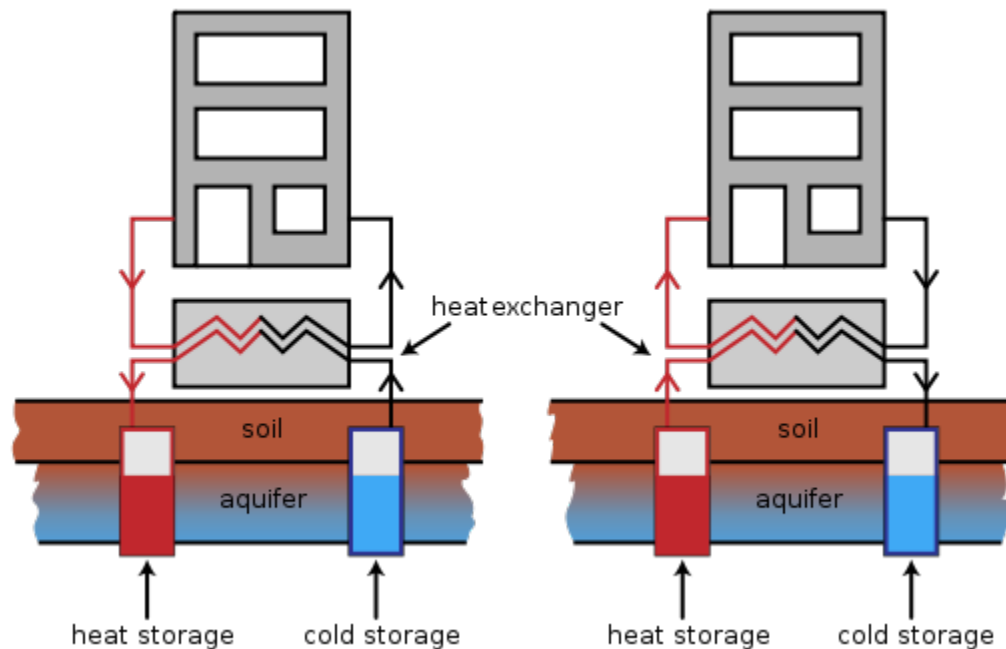
A heat pump in combination with heat and cold storage
