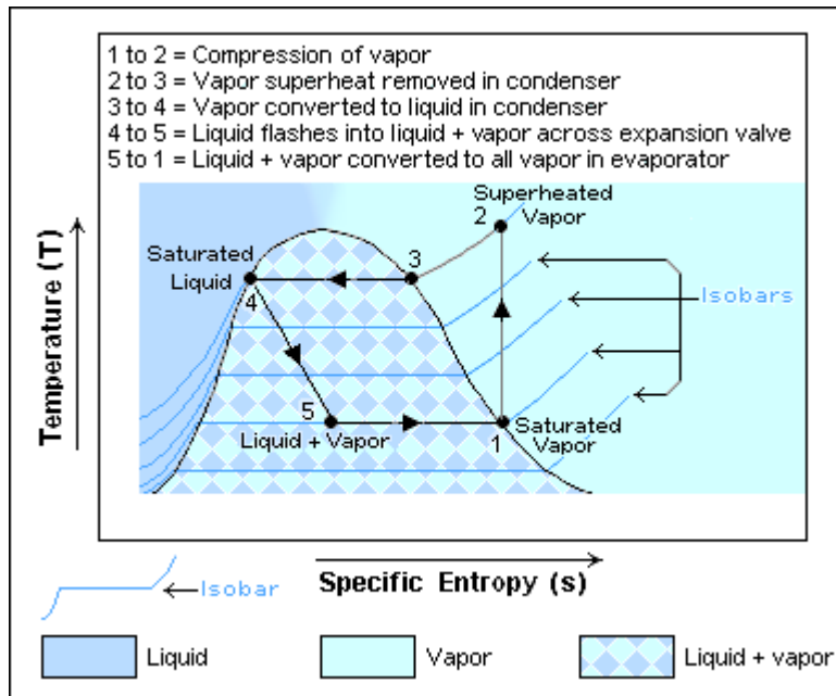
Figure 2: Temperature-Entropy diagram
