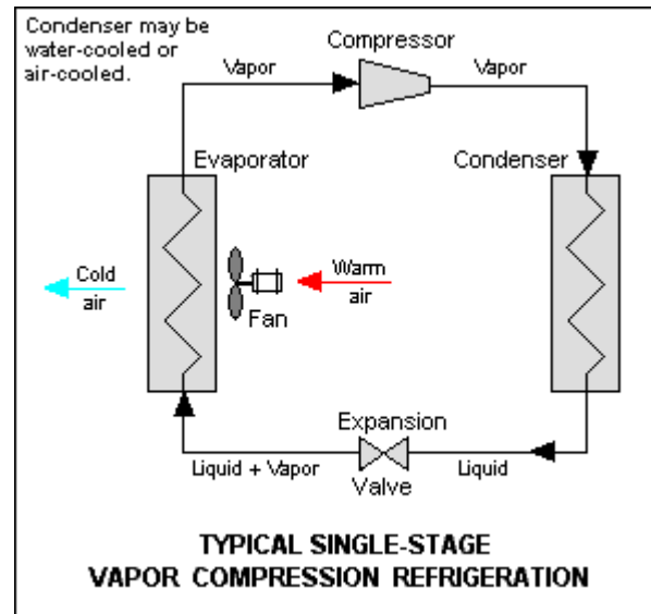
Figure 1: Vapor compression refrigeration
