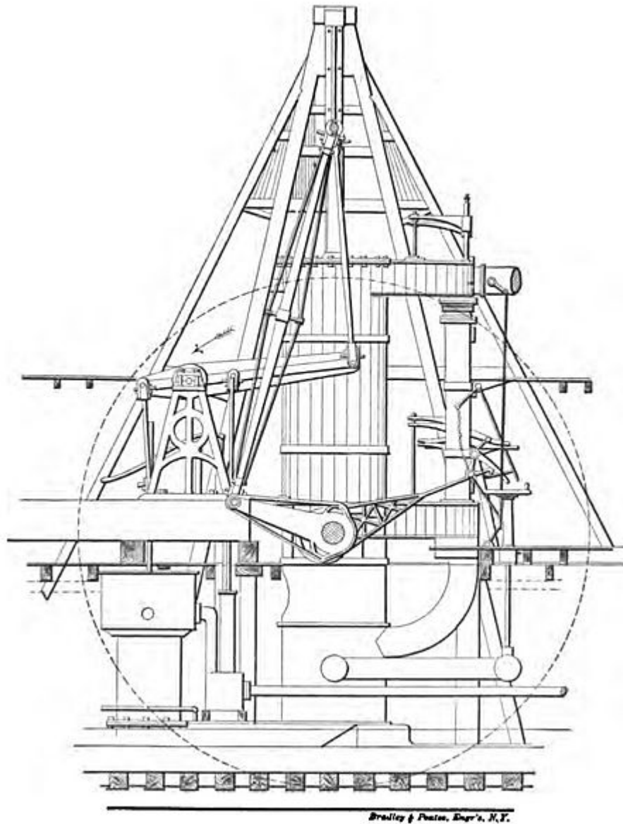
Diagram of a typical Hudson River steamboat crosshead engine (side view)
