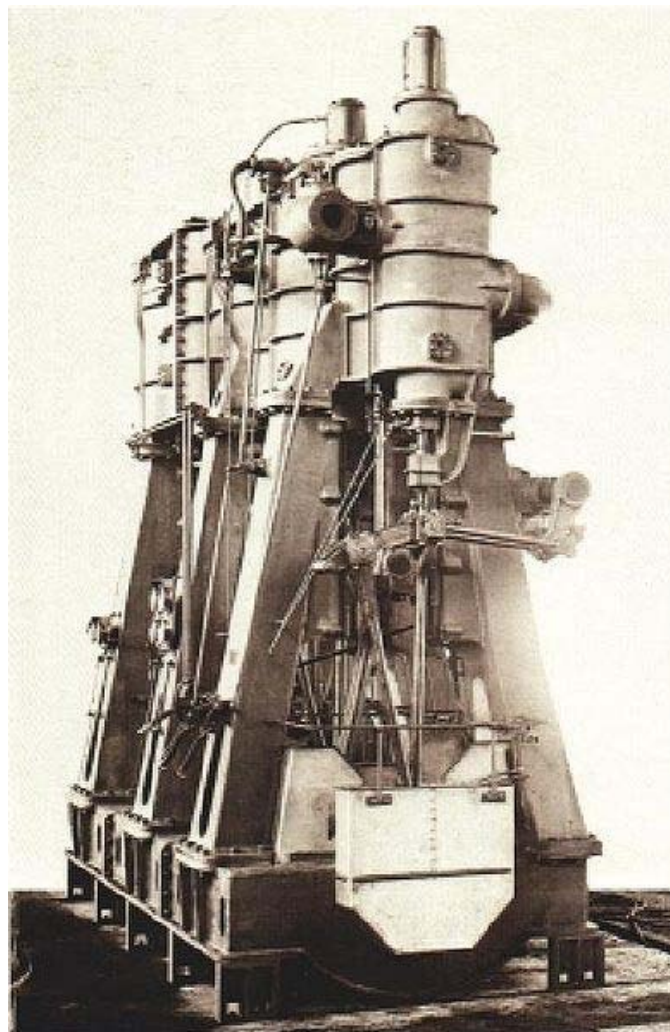
A Joshua Hendy triple expansion engine
