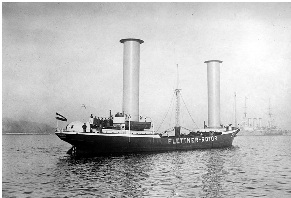
Rotor ship Buckau
