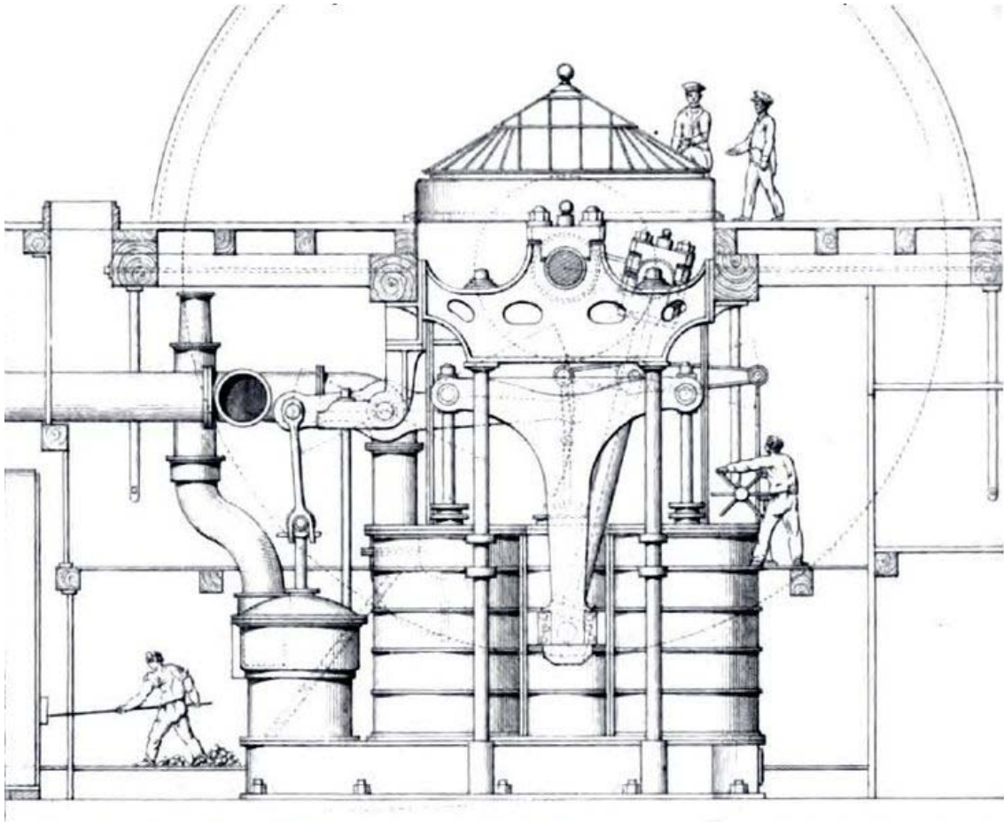
Siamese engine of HMS Retribution (1844)
