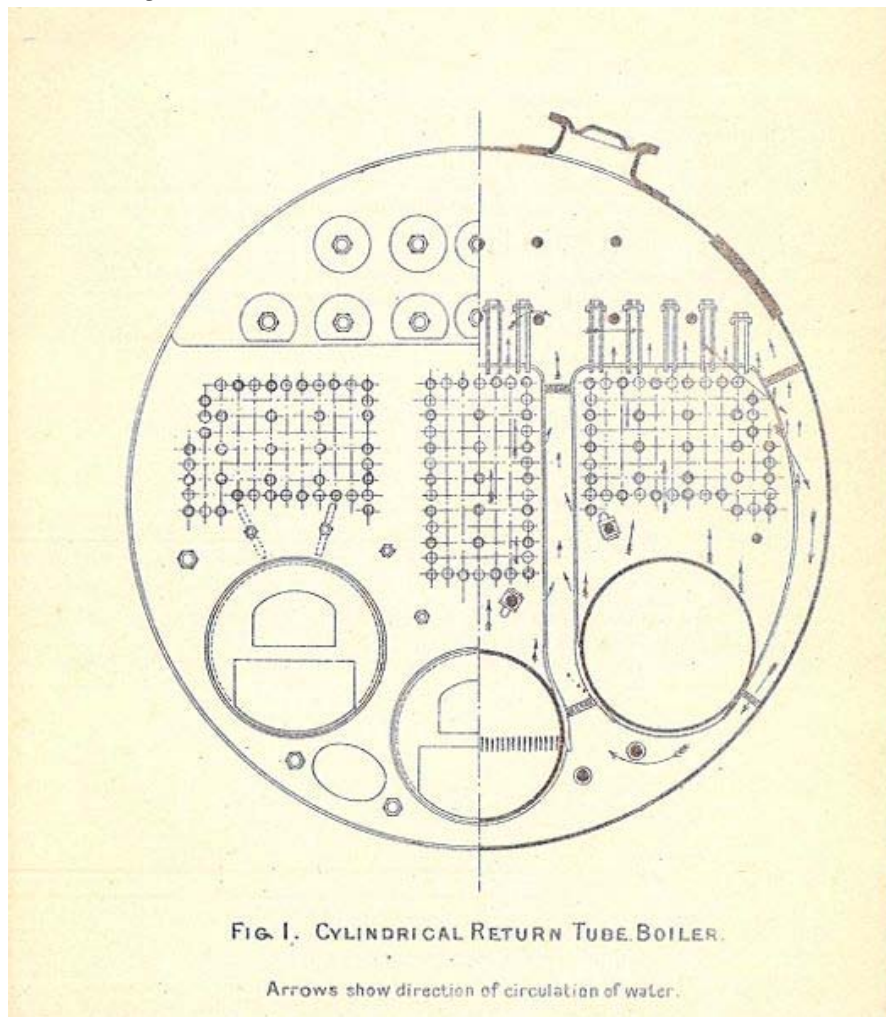
End view and half-section of a three-furnace boiler
