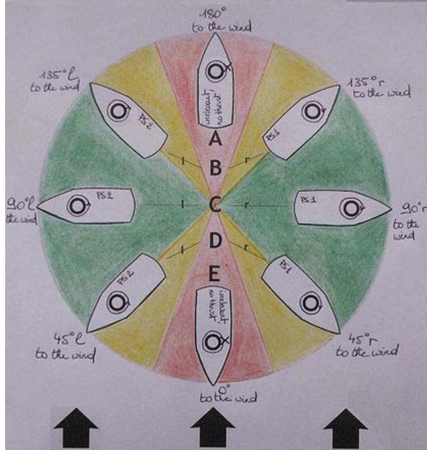
The points of sail for a rotorship
