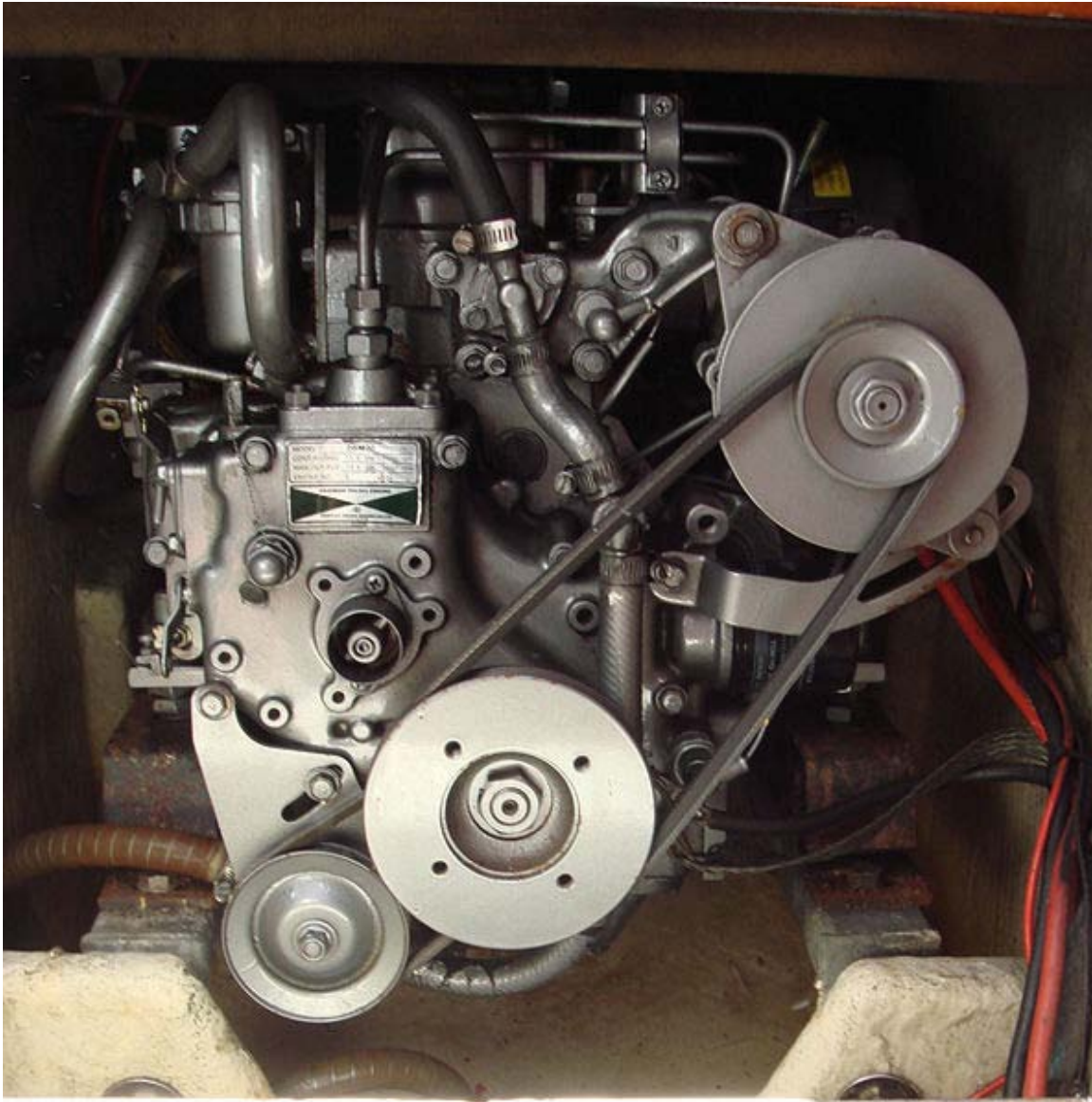
A Yanmar 2GM20 inboard marine diesel engine, installed in a sailboat.
