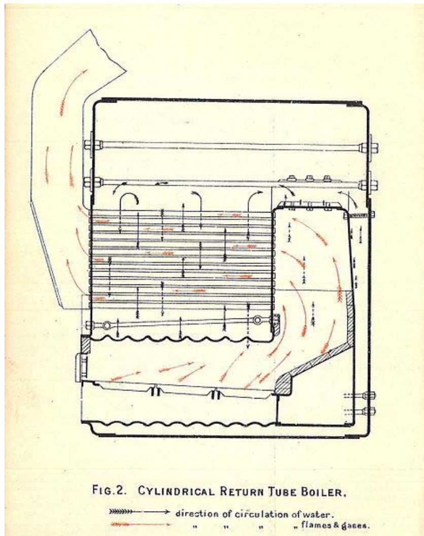
Sectional diagram of a "wet back" boiler
