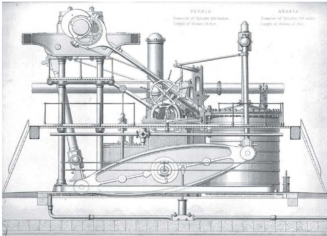
Side-lever engine of RMS Persia (1855)
