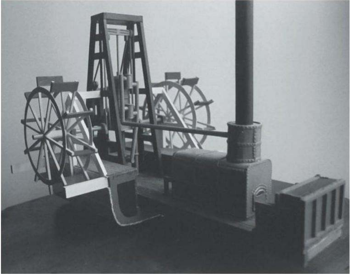
Model of a crosshead or "square" engine, showing location of engine cylinder above the crankshaft; also piston rod, crosshead, connecting rods and paddlewheels
