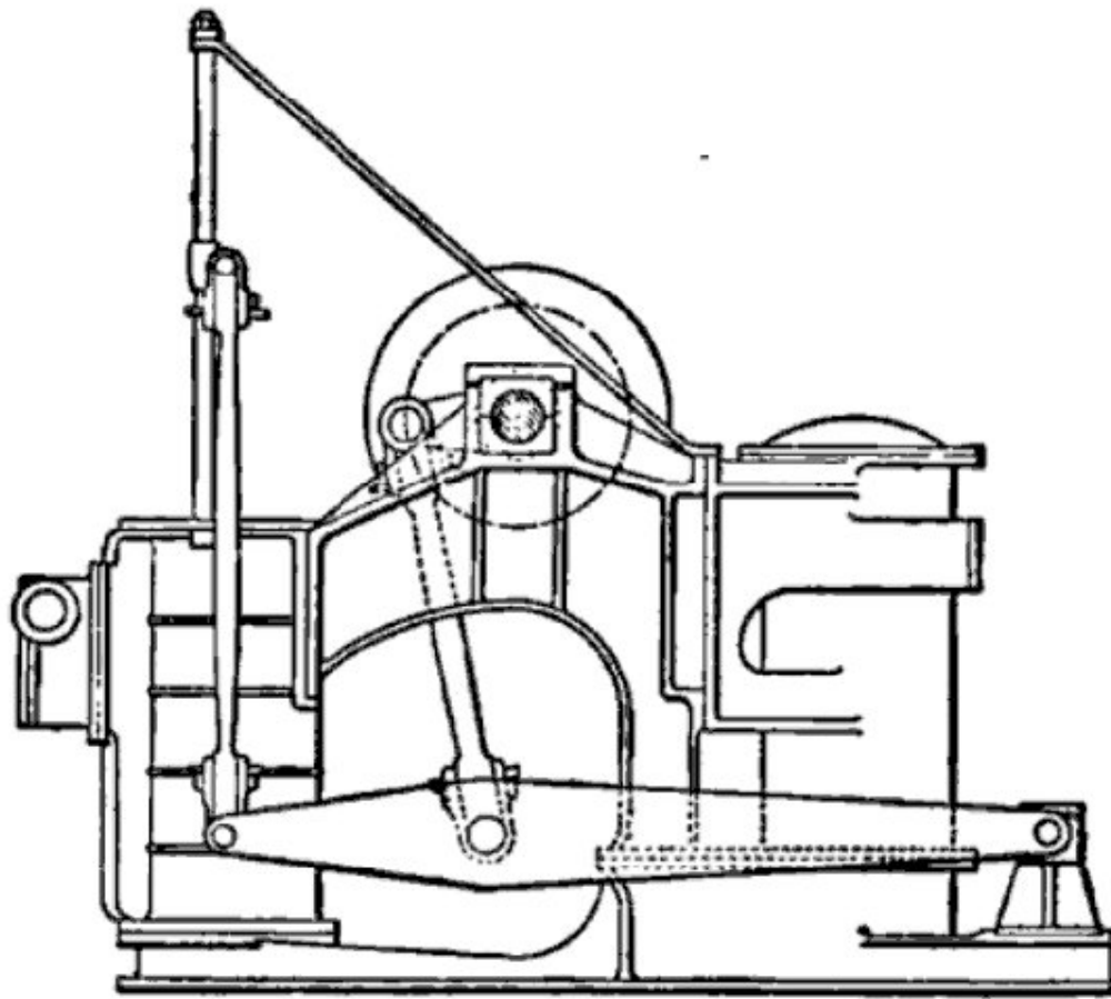
Fig. 3. — "Grasshopper" Engine.
