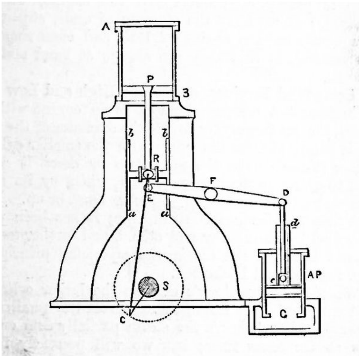
Diagram of a simple "hammer" engine
