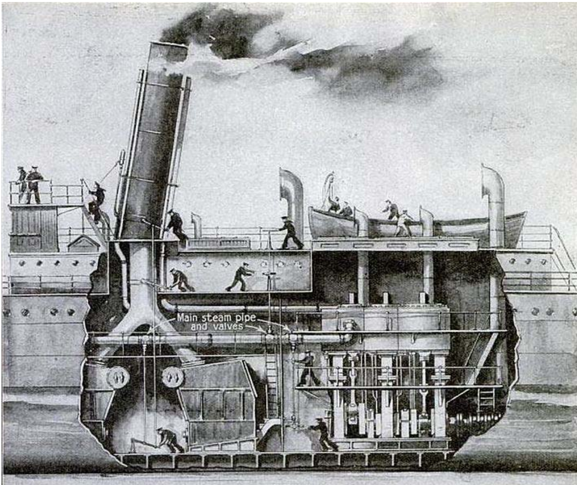
Period cut away diagram of a triple expansion steam engine installation, circa 1918
