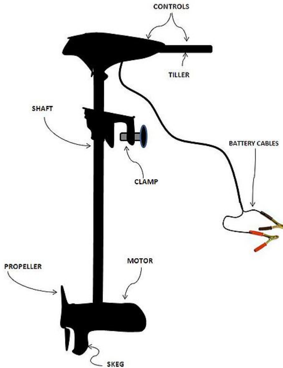
Diagram of a hand-controlled trolling motor.
