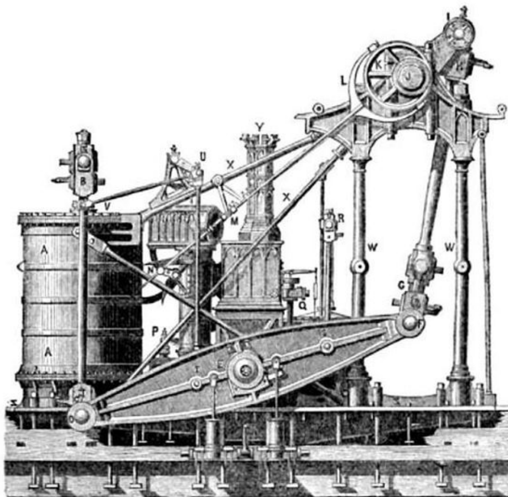
FIG. 92.—The Side-Lever Engine, 1849.
