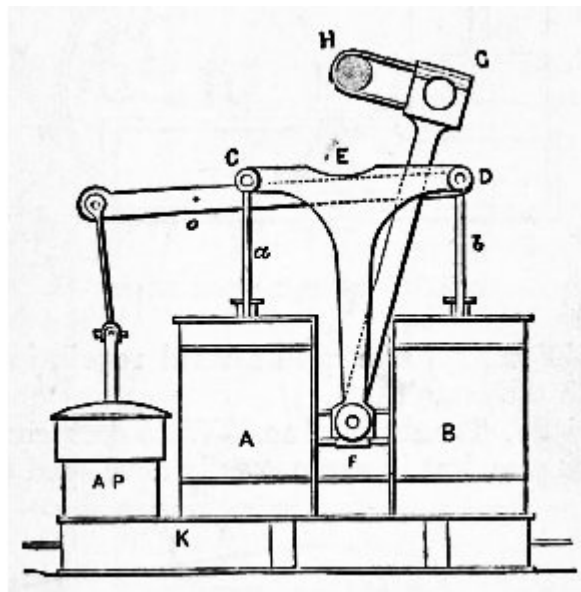
Basic diagram of a Siamese engine
