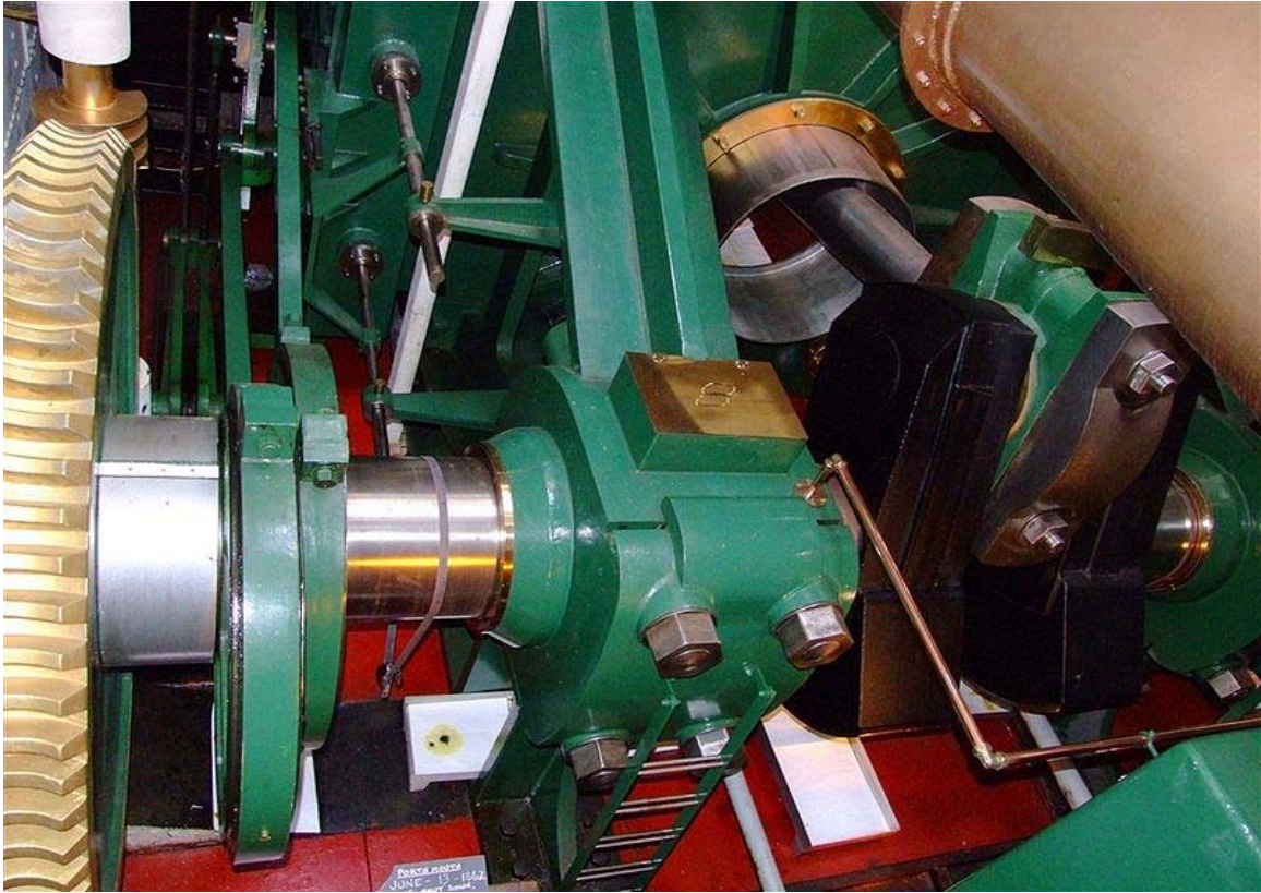
Looking down at the trunk engine of HMS Warrior (1860). The connecting rod can be seen emerging from the trunk at right.
