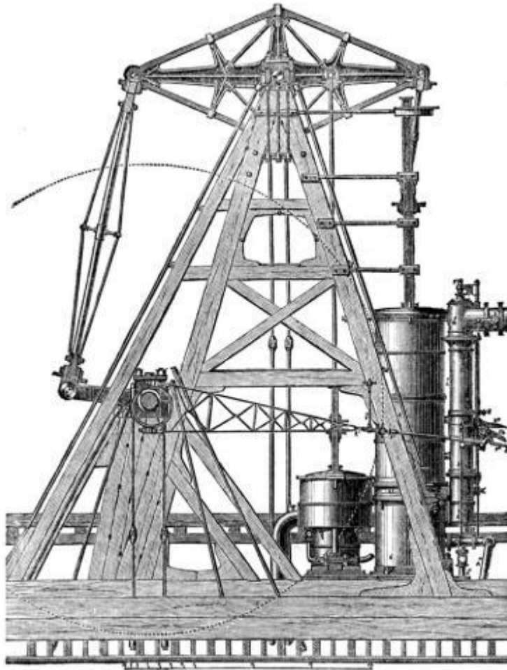
FIG. 180.—Beam-Engine.
