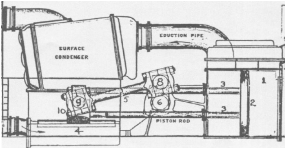
Diagram of back-acting engine of USS Ranger
