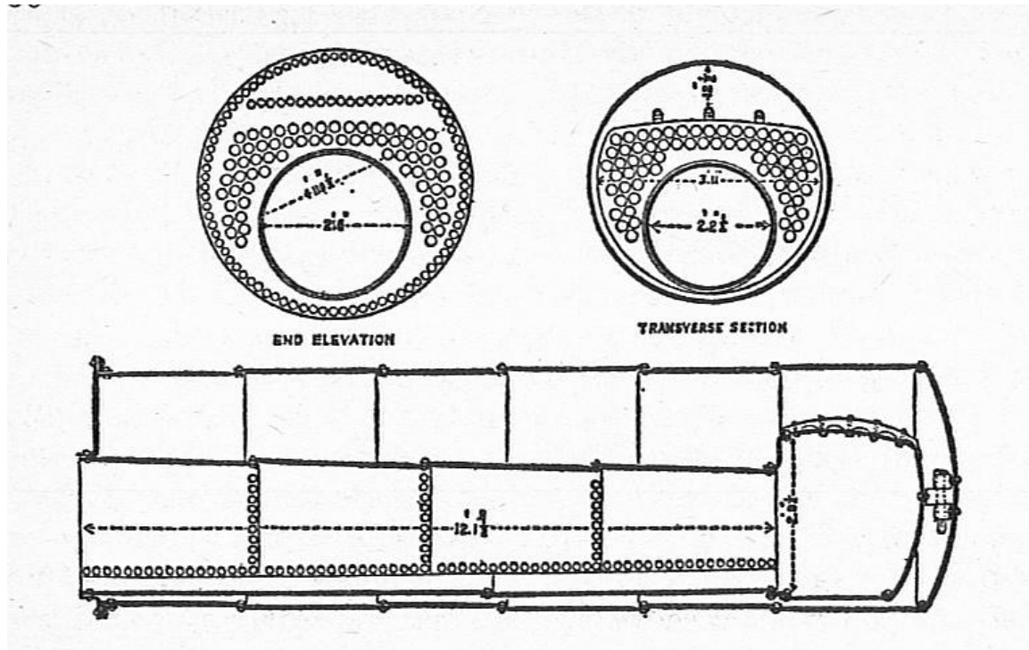
'Wilberforce' boiler in section
