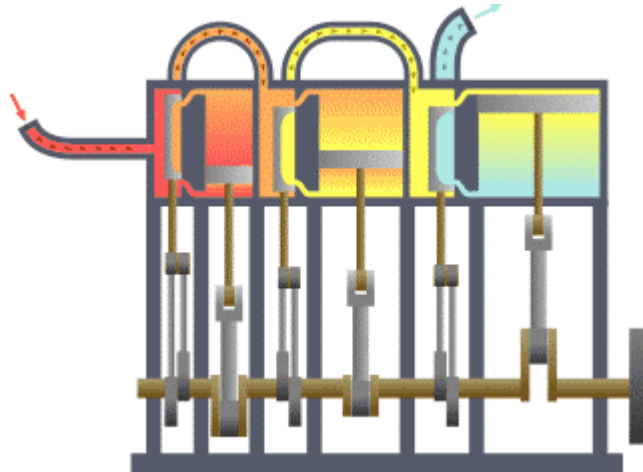
A typical vertical triple-expansion engine
