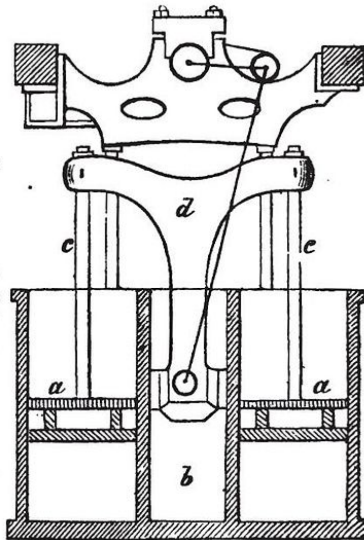
Annular Engine.
