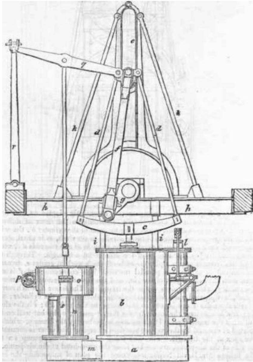
Steeple engine
